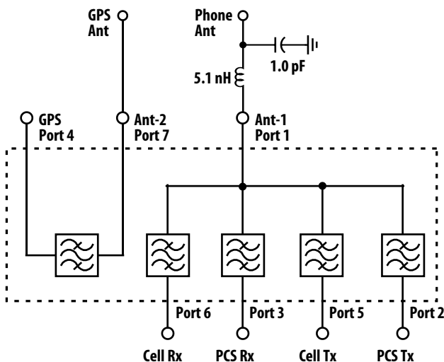
Figure 1. Dual Antenna Application.
