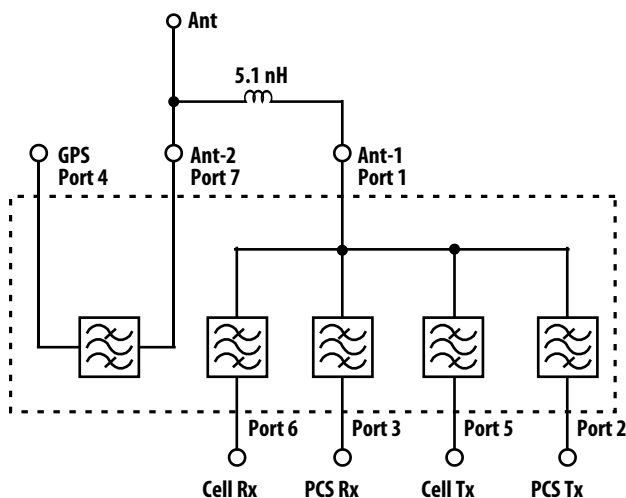
Figure 2. Single Antenna Application.
