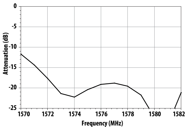
Figure 31. Antenna Port Return Loss in GPS Band (Dual Antenna, Note1).
