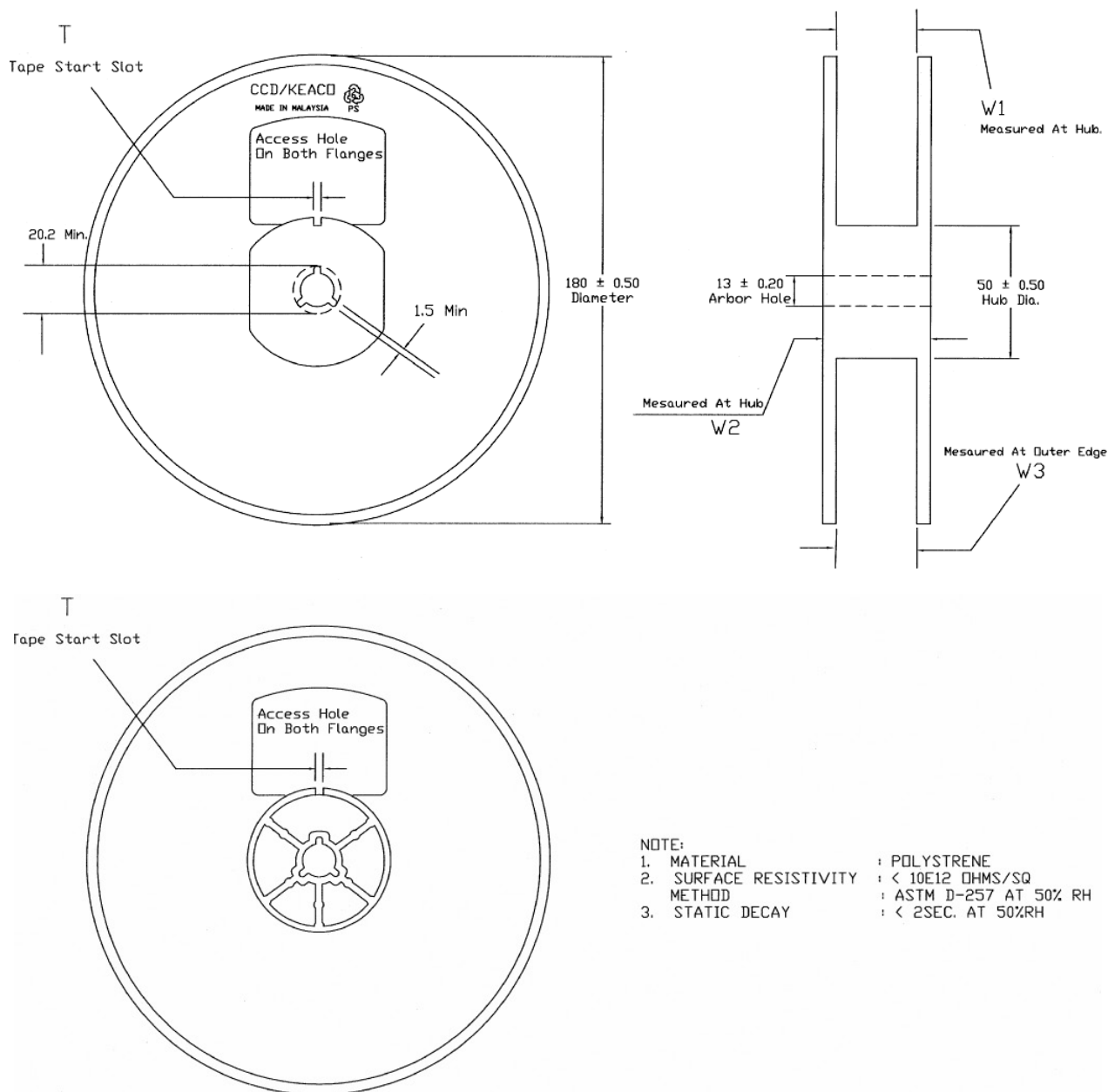
Figure 54. Reel Drawing
