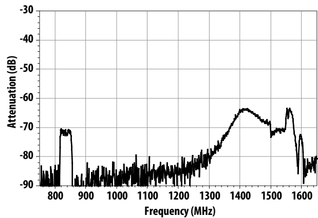
Figure 32. Cellular Tx Port to GPS Port Isolation (Dual Antenna, Note1).
