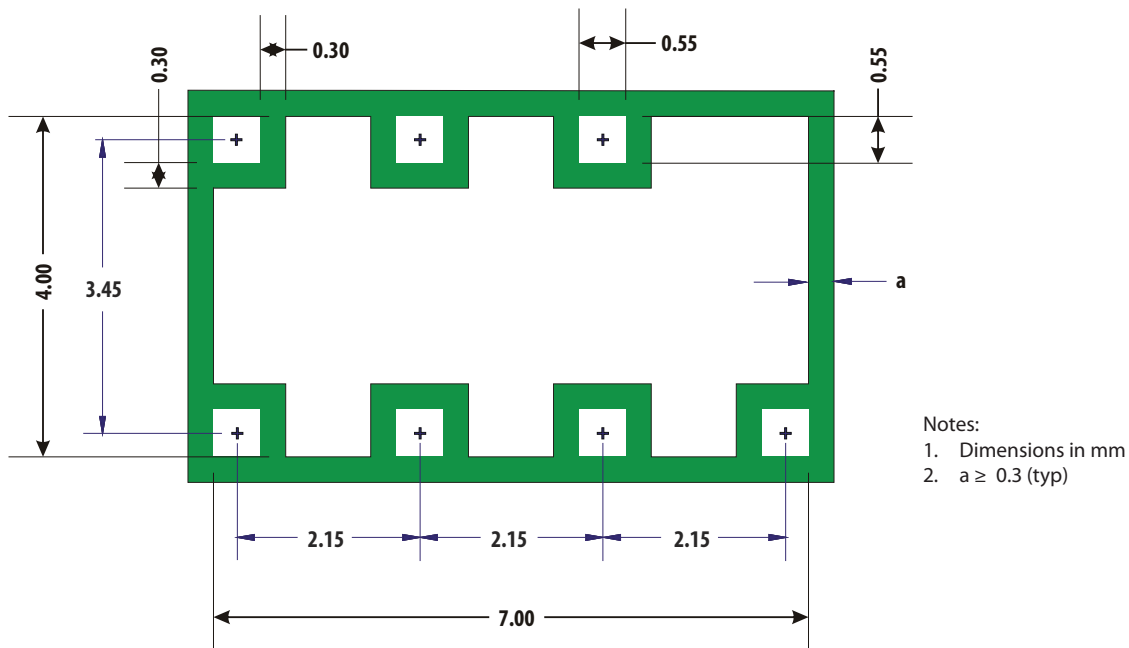
Figure 45. Recommended Solder Mask (top view).
