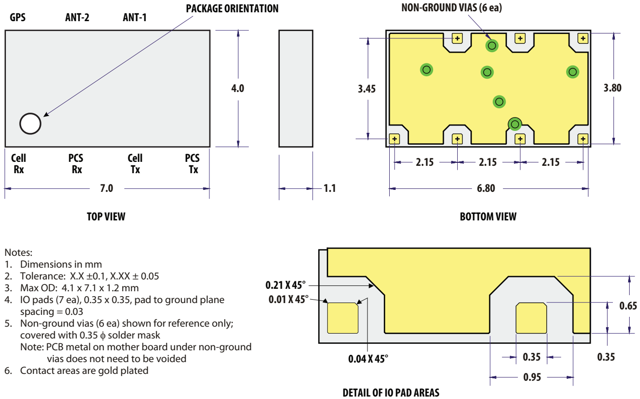
Figure 39. Package Outline Drawing.
