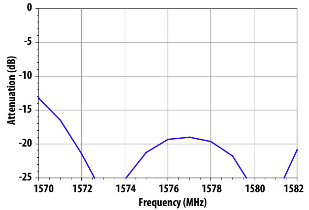
Figure 30. GPS Port Return Loss (Dual Antenna, Note1).
