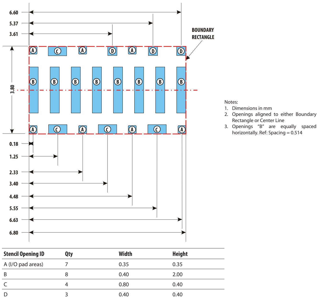
Figure 46. Recommended Solder Stencil (top view).
