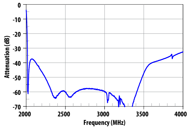
Figure 14. PCS Ant-Rx Rejection, 2000-4000 MHz (Dual Antenna, Note1).
