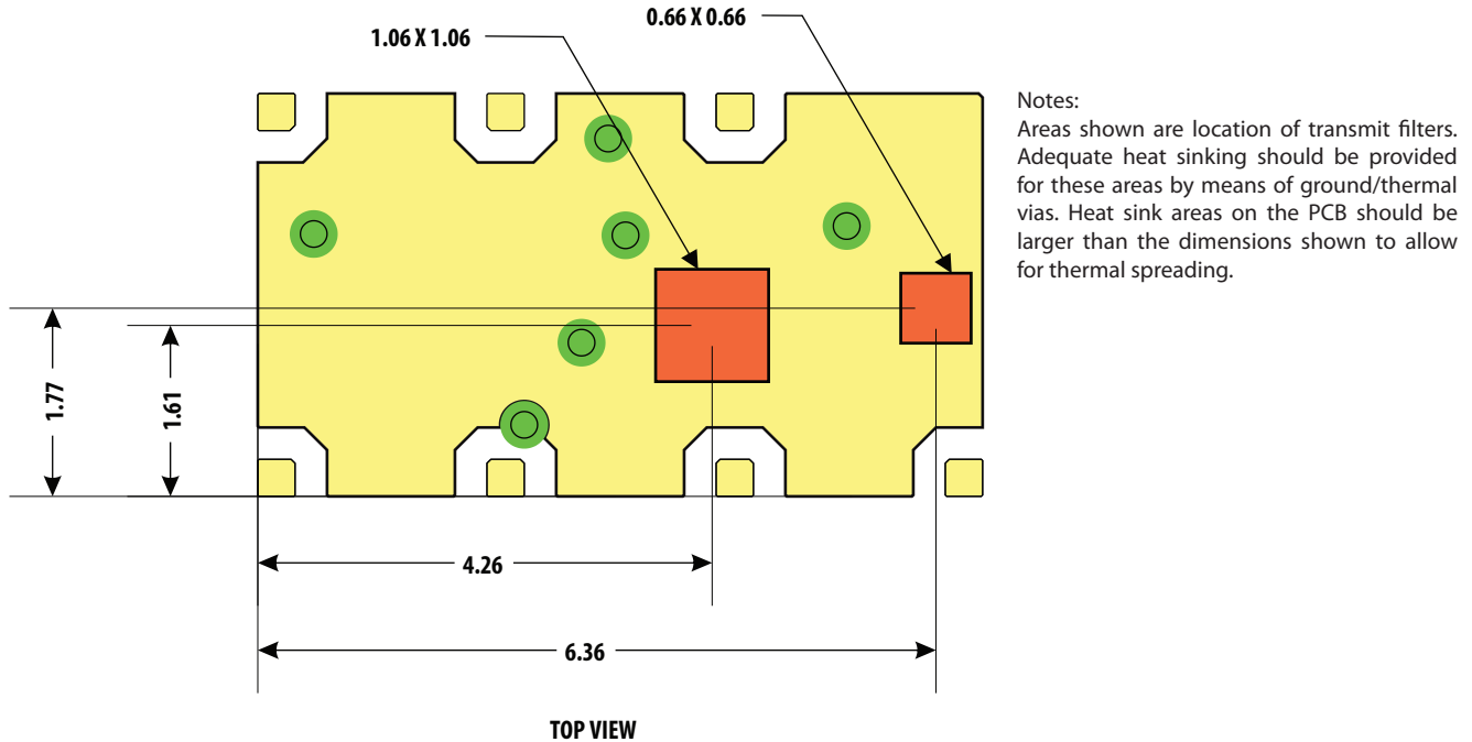
Figure 44. Location of Heat Sink Areas (top view).
